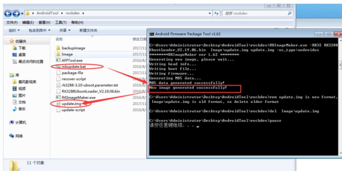
Figure 4-3 Script-to-generate-images
